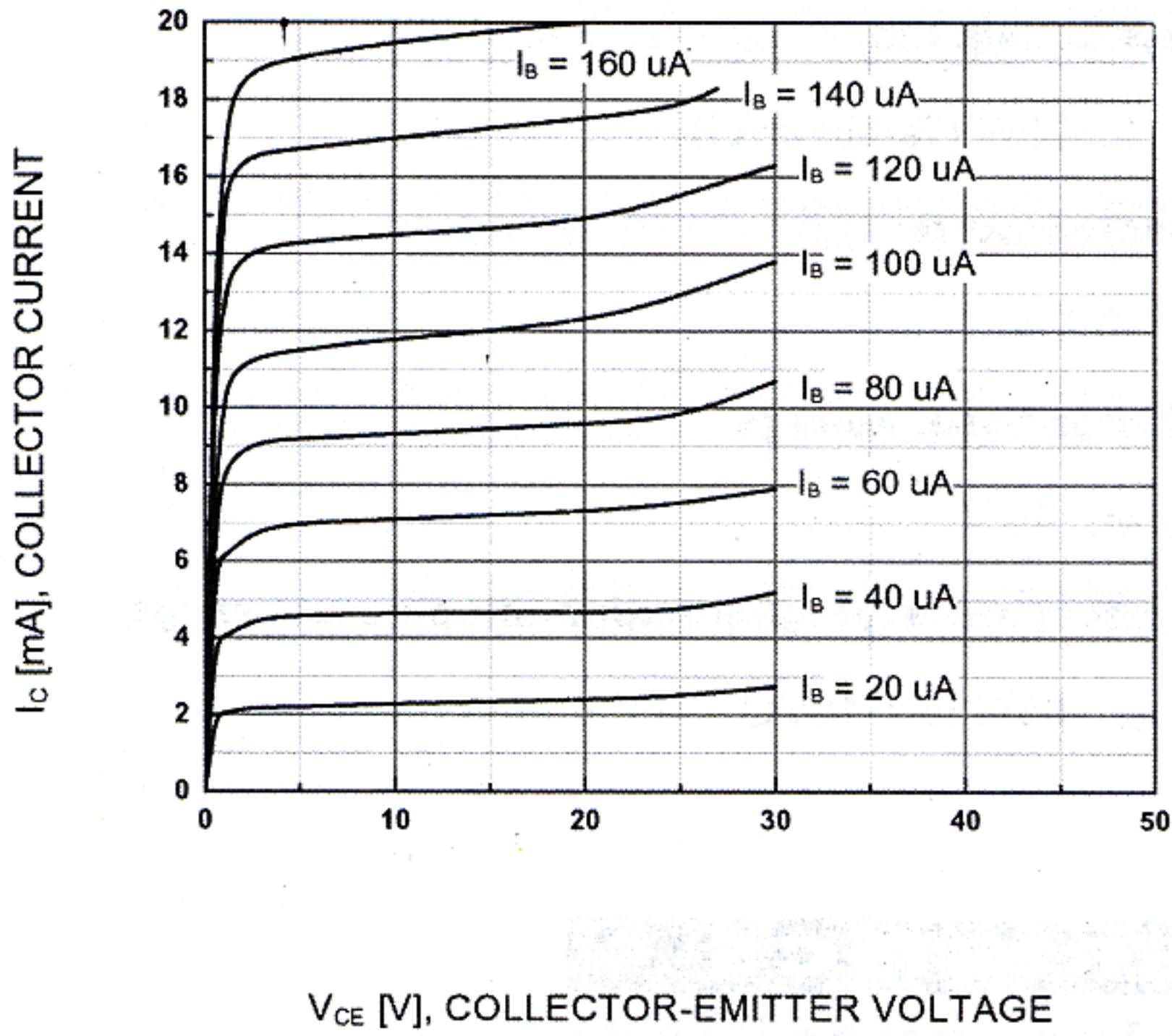
Static Characteristic
