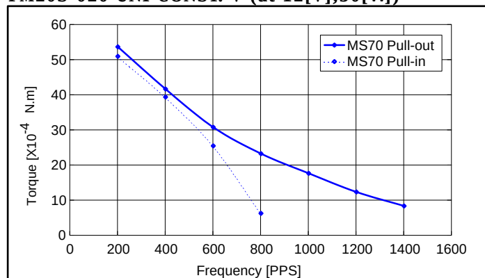
PM20S-020 UNI-CONST. V (at 12[V],50[W])
