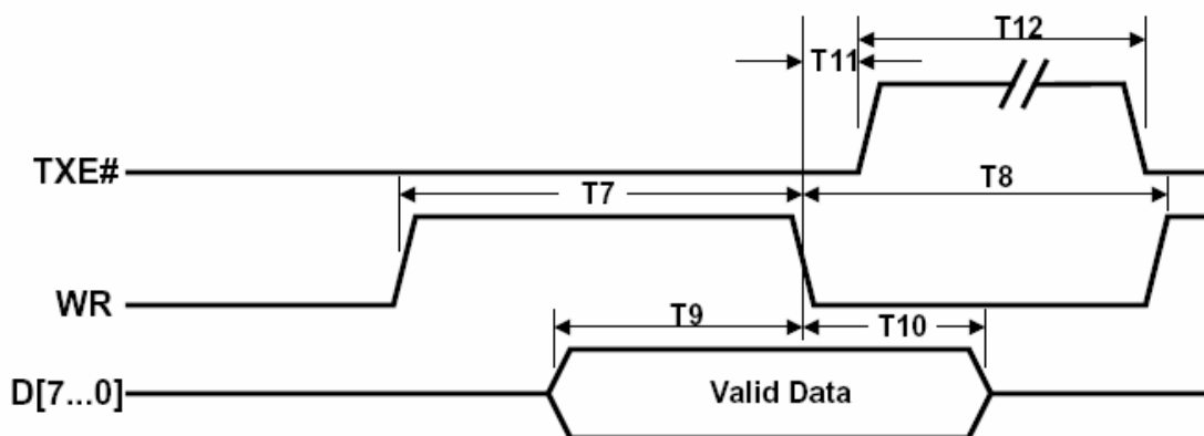
Image for FT245R FIFO Write cycle taken from the FT245R datasheet.
