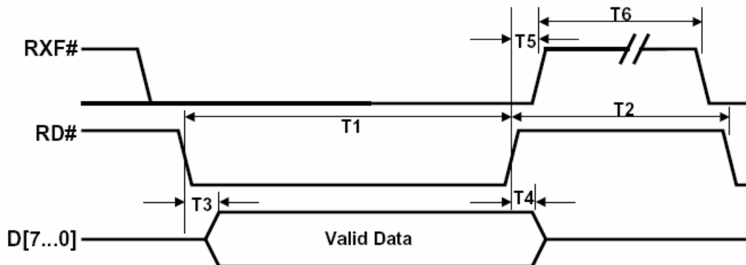
Image for FT245R FIFO Read cycle taken from the FT245R datasheet.
