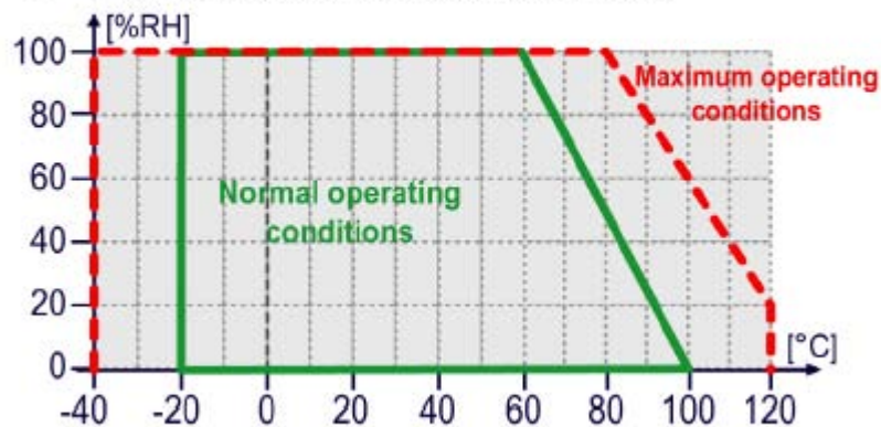
Figure 11 Recommended operating conditions
