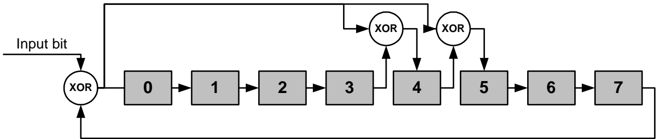
Figure 1 Internal structure of the FOSTxx CRC-8 generator
