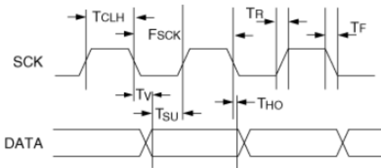
Figure 9 Timing Diagram
