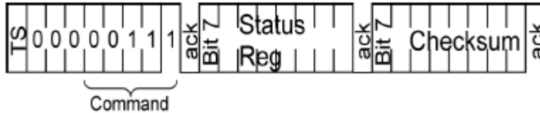
Figure 8 Status Register Read
