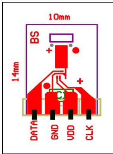
DIP package
