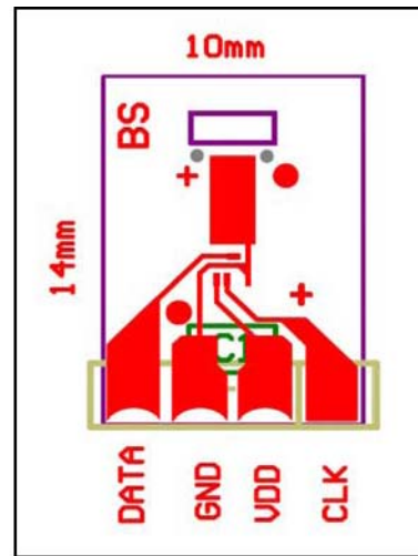
SMD package
